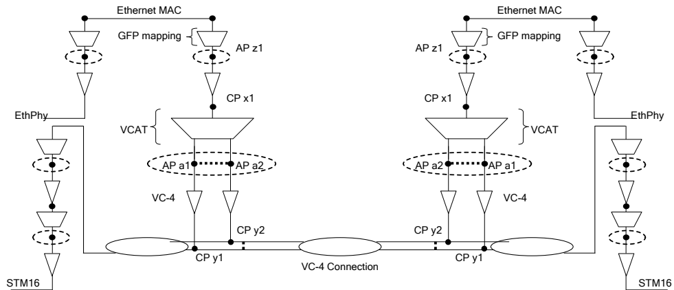
Figure 6. G.805 drawing showing EthMac and VC4 layer relationship
