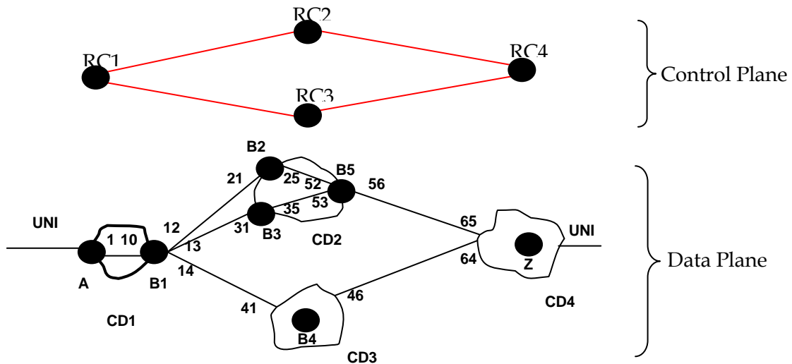
Figure 13: Example Topology
