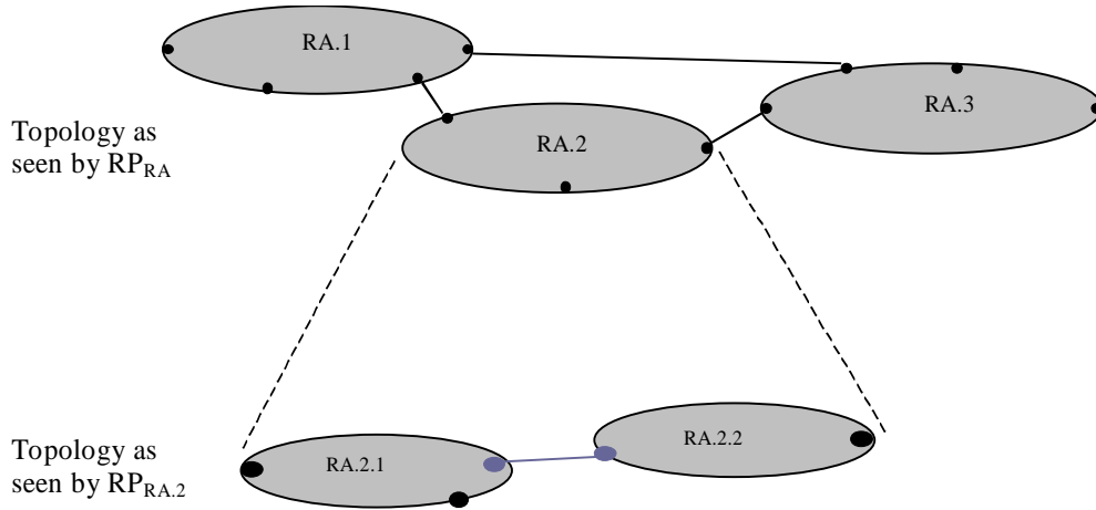
Figure 15: Topology Views as Seen by RP Associated with Hierarchical Routing Areas (Figure 7 in [G.7715])
