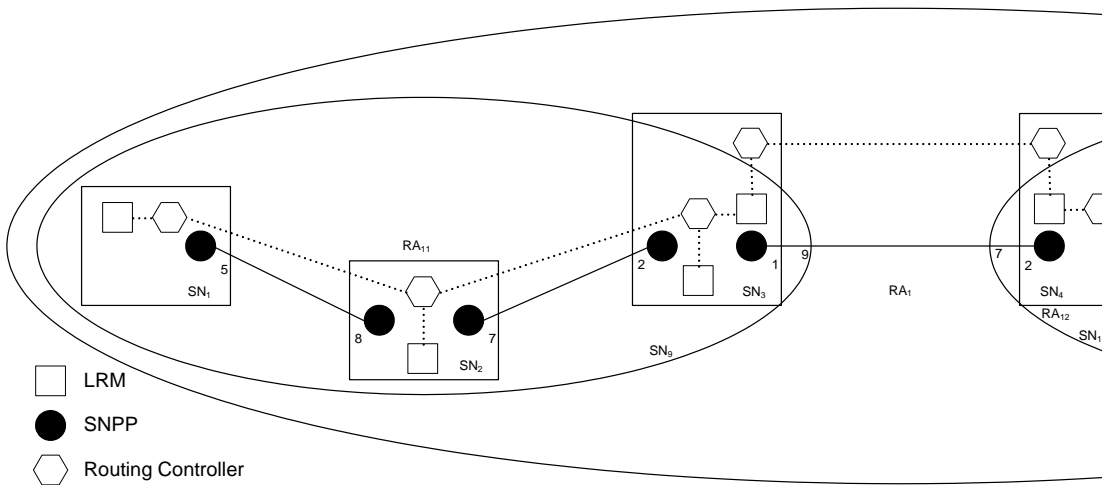
Figure 16: Hierarchical Routing Controller Relationships
