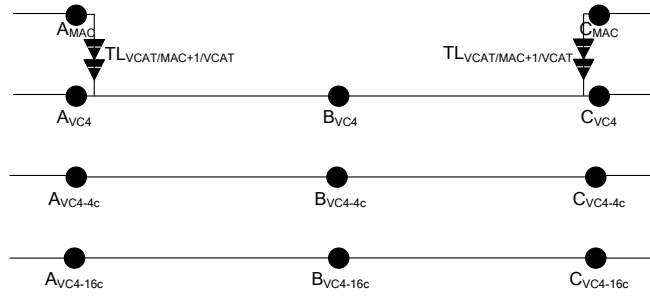
Figure 7. Link-oriented Routing Topology showing EthMac/VCAT Transitional Link
