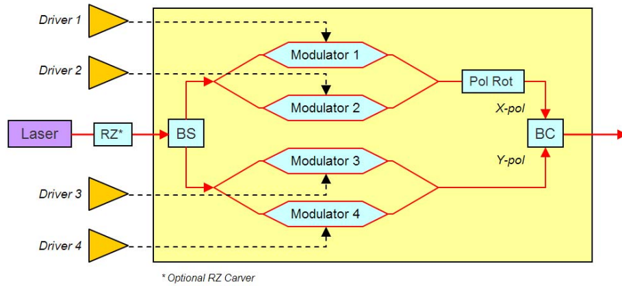
Figure 4. Block diagram of a DP QPSK transmitter module
