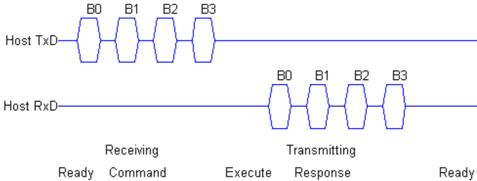
Figure 7.2-1: RS232 Timing
