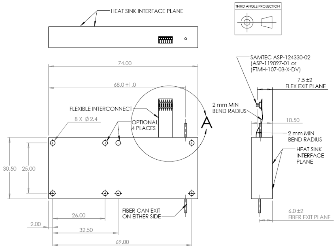
Figure 12.1-1: Mechanical Outline Dimensions
