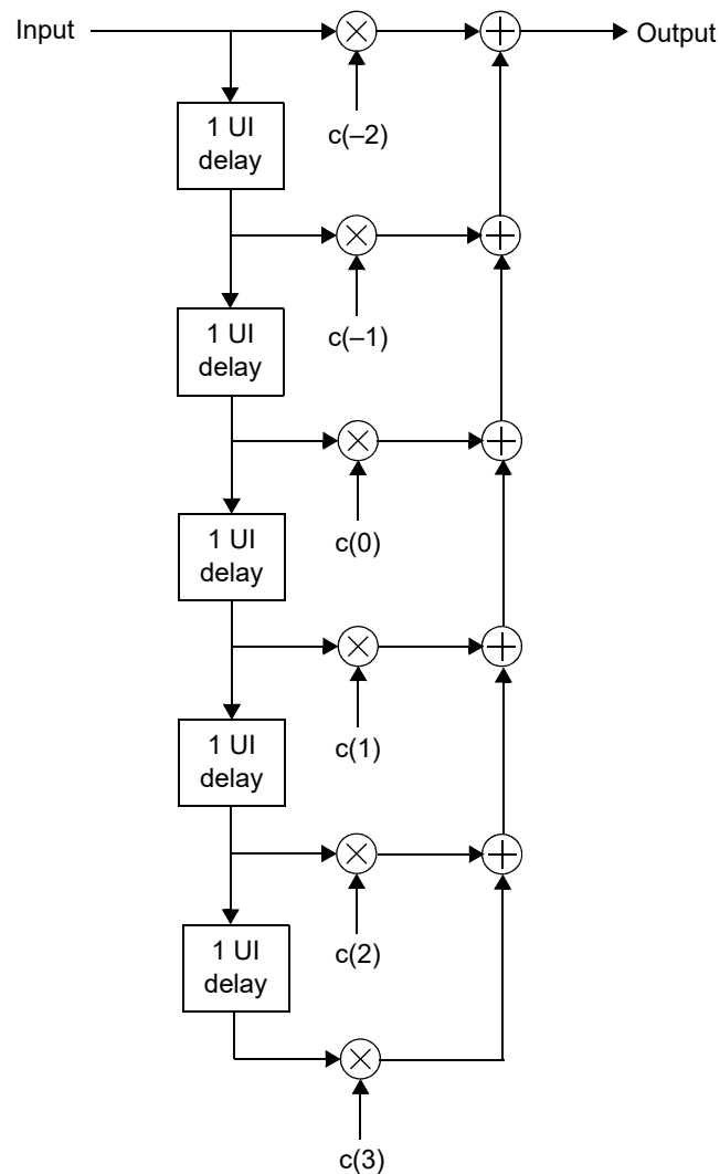
Figure 28-3. Transmit equalizer functional model
