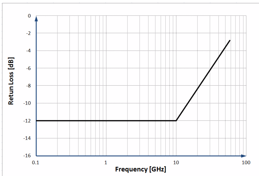
Figure 18-5. Illustration of Return Loss for T_{\text{Baud}} = 58.0 \text{ Gsym/s}
