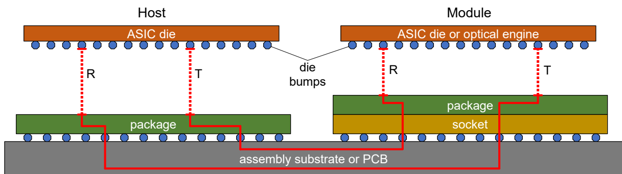
Figure 28-1. Reference Model for Channel with socket
