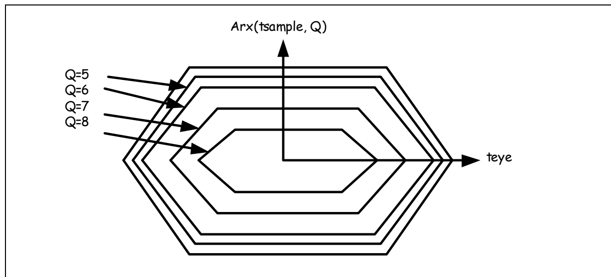
Figure 2-23. Statistical Eye
