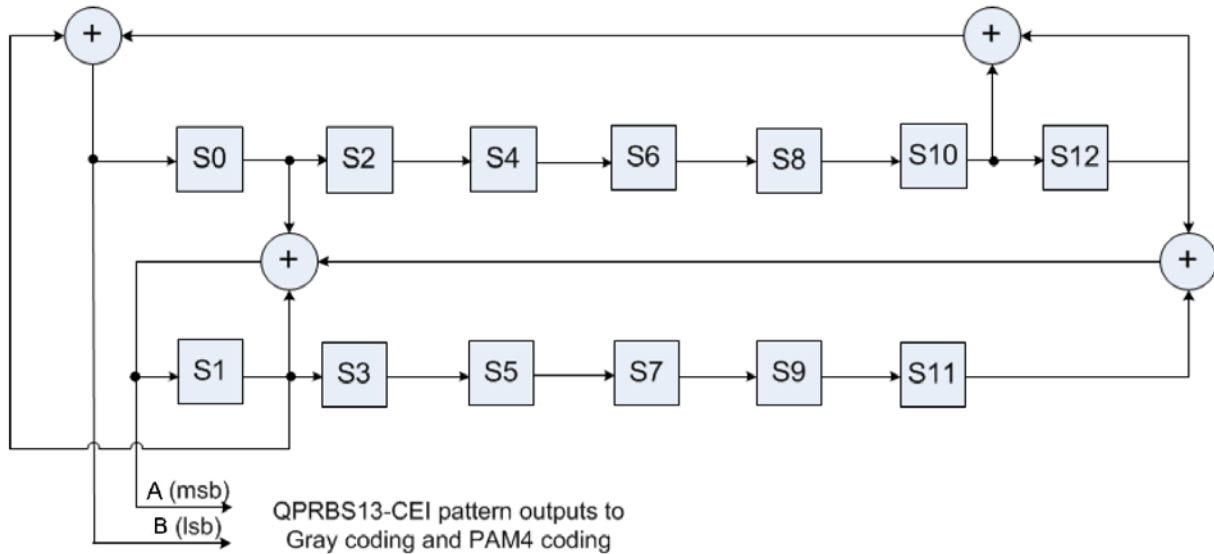
Figure 16-19. QPRBS13-CEI pattern generator
