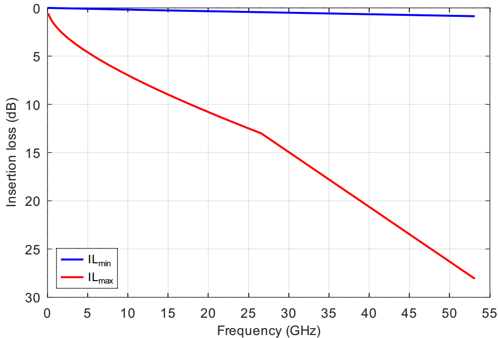
Figure 28-2. Channel Insertion Loss Limits for 53.125 Gsym/s
