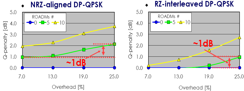
Figure 3 Impact of ROADM impairment in absence of equalizer.
