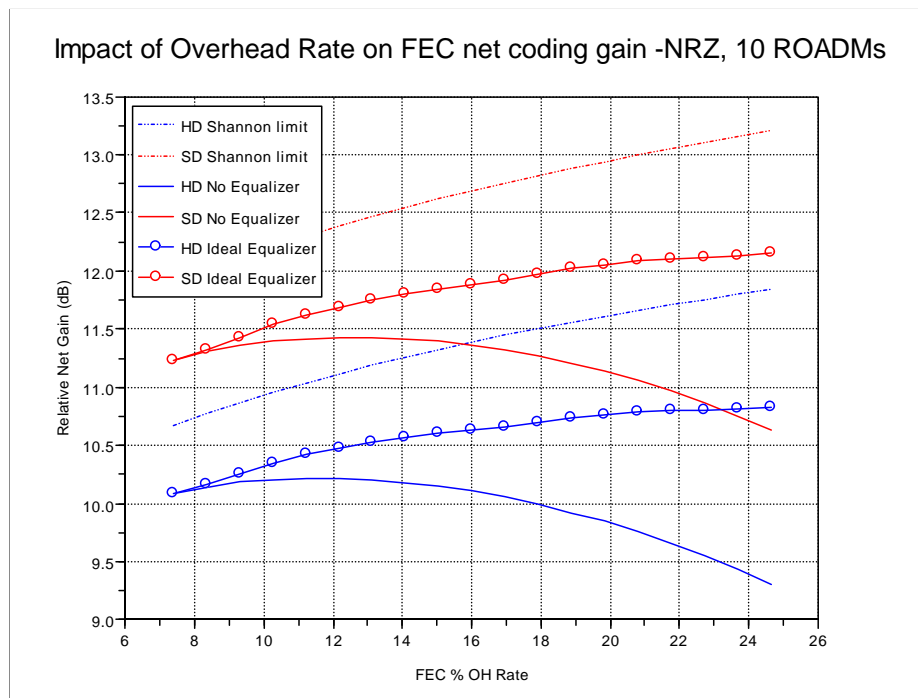
Figure 6 Relative NCG with and without equalization for NRZ
