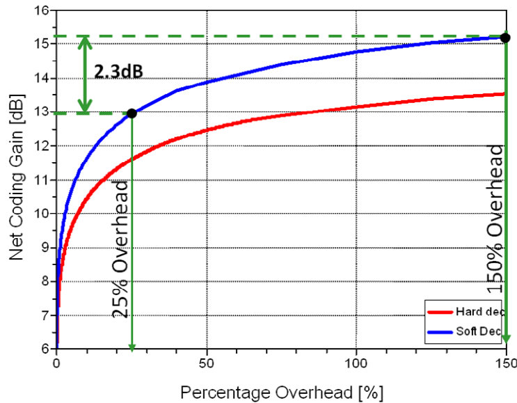
Figure 2: The Shannon Limit - Maximum Theoretical NCG [Cai 05]
