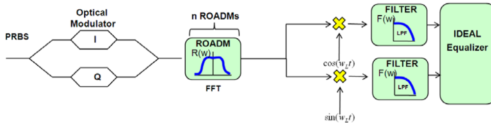
Figure 5 Simplified Link Model
