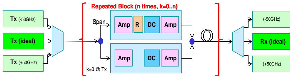
Figure 4 Generic Link Model
