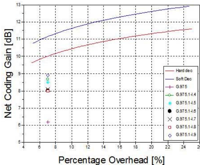
Figure 1 Comparison of NCG for Standardized FECs against the Shannon Limits
