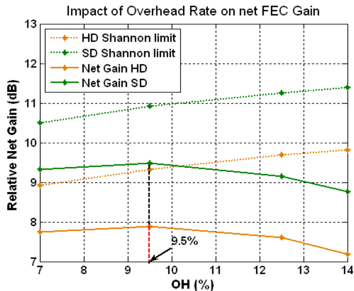
Figure 7 Net coding gain versus percentage overhead with equalization for NRZ for a particular scenario.
