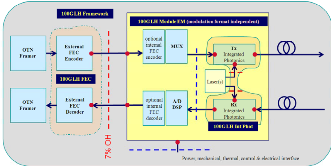
Figure 8 100G DP-QPSK Transceiver module functional architecture with enhanced FEC.
